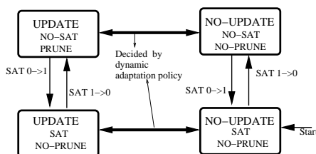
Fig. 4: State machine for dynamic adaptation mechanism
