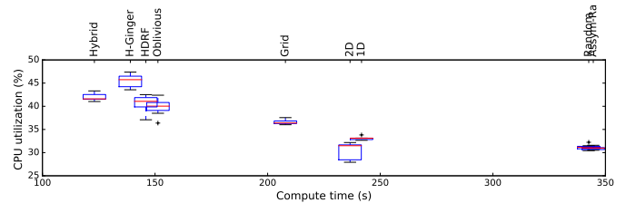
(a) PageRank
